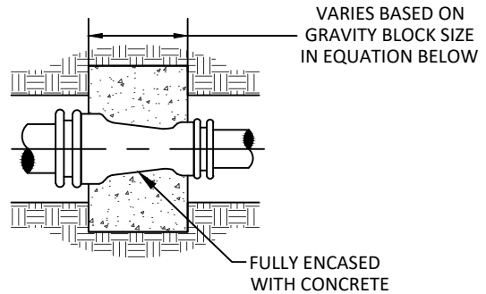
REDUCER
