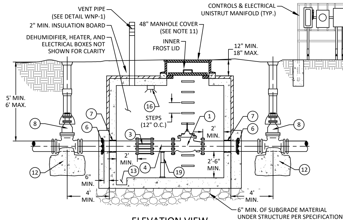
ELEVATION VIEW
