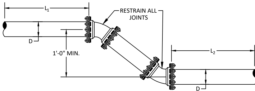
VERTICAL OFFSET
