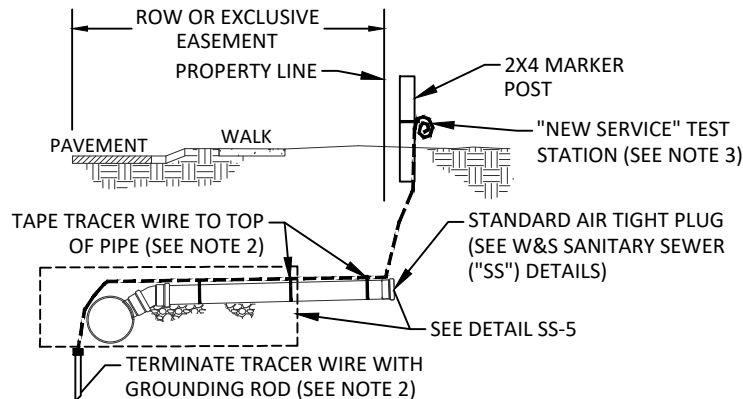
TRACER WIRE INSTALLATION - NEW CONSTRUCTION
