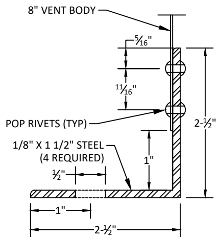
STEEL ANGLE DETAIL
