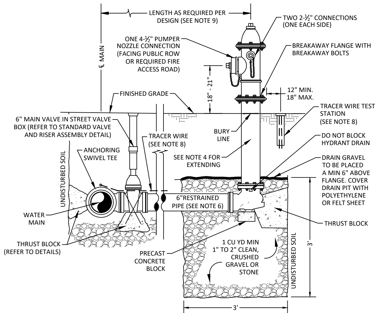
ELEVATION VIEW
