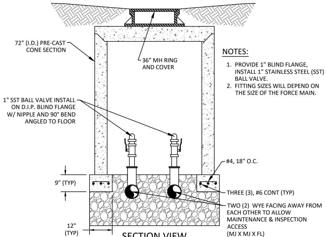
SECTION VIEW
