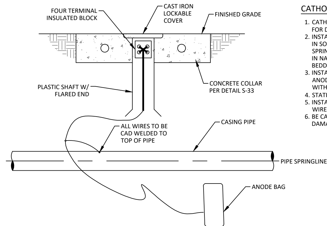
CATHODIC TEST STATION DETAIL
