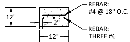
BASE BEAM DETAIL
