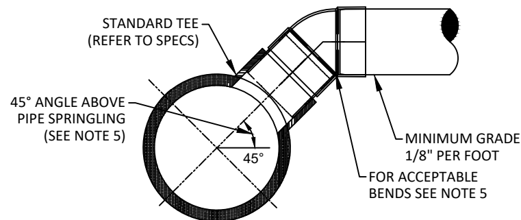
STANDARD TEE CONNECTION
