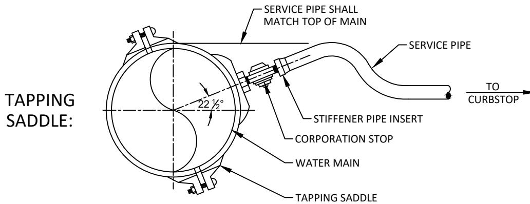
ELEVATION VIEW
