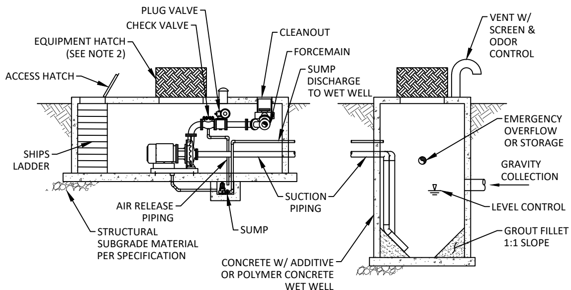
SECTION VIEW
