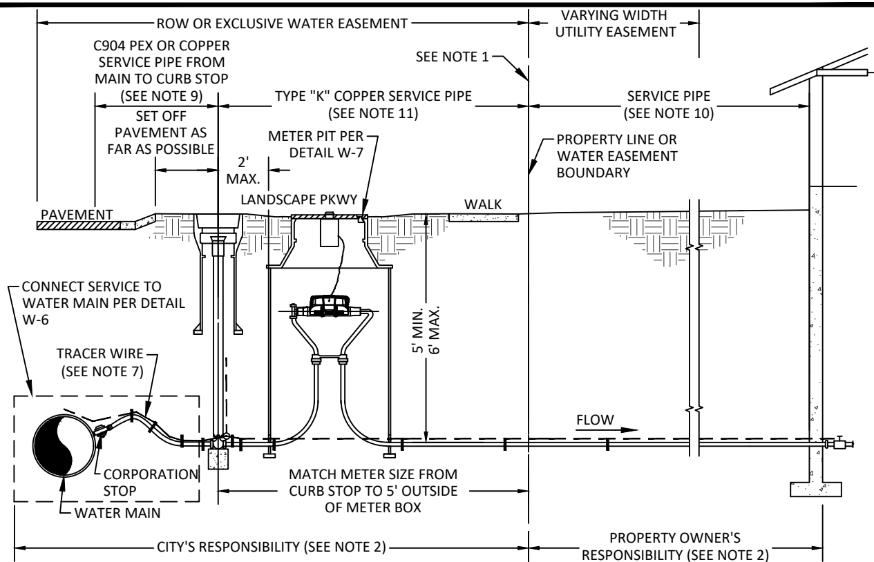
ELEVATION VIEW
