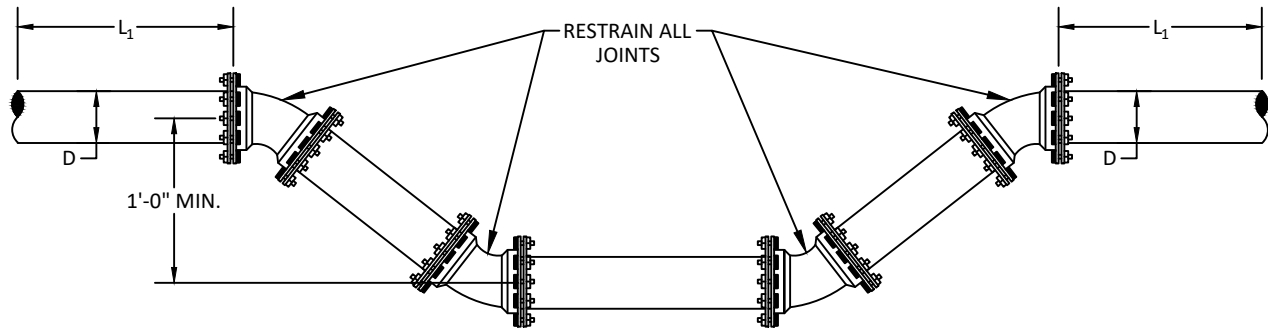
VERTICAL LOWERING
