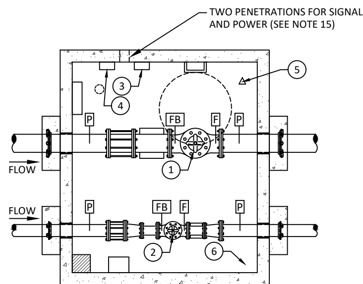
PLAN VIEW (TYP.)
